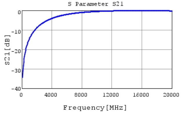
GRM0335C1HR30BA01 S21 DCOV, 25degC
