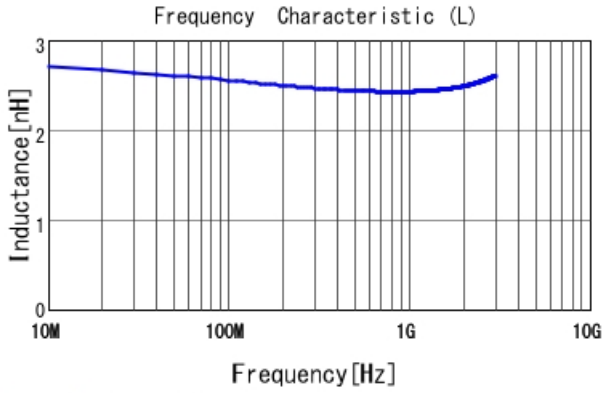
LQP03TN2N4C02 L
