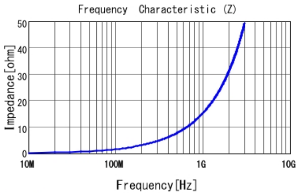
LQP03TN2N4C02 |Z|
