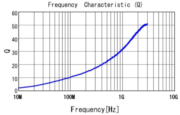
LQP03TN2N4C02 Q
