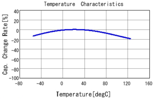
GRM31CC72A475KE11 C-Temp. capchange, DC0.0V, ACO.1
