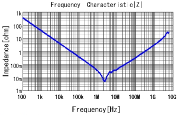
GRM31CC72A475KE11 |Z| DCOV, 25degC
