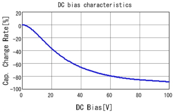
GRM31CC72A475KE11 C-DC bias capchange, 25.0degC, A
