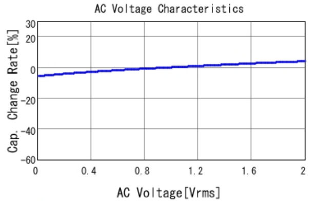
GRM31CC72A475KE11 C-AC Voltage capchange, DCOV, 25
