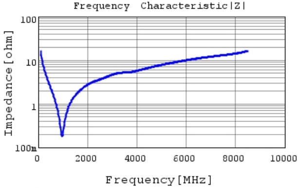
GRM0335C1H101JA01 |Z| DCOV, 25degC
