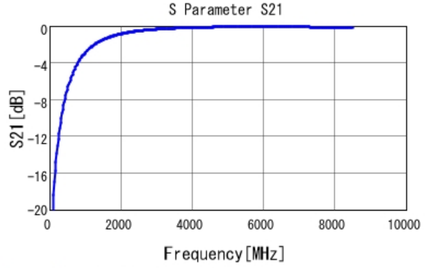
GRM1555C1H1R6BA01 S21 DCOV, 25degC
