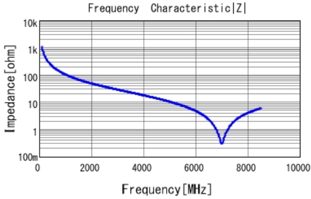
GJM1555C1H1R5WB01 |Z| DCOV, 25degC
