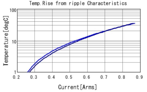
GJM1555C1H1R5WB01 Temp. rise — 2GHz — 3GHz
