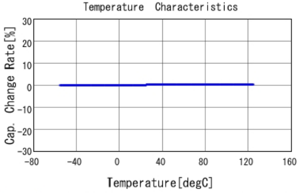
GJM1555C1H1R5WB01 C-Temp. capchange, DCOV, AC1Vrms
