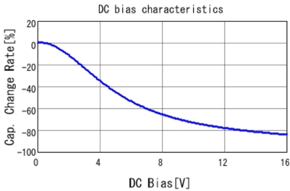
GRM185R61C105KE44 C-DC bias capchange, 25.0degC, A
