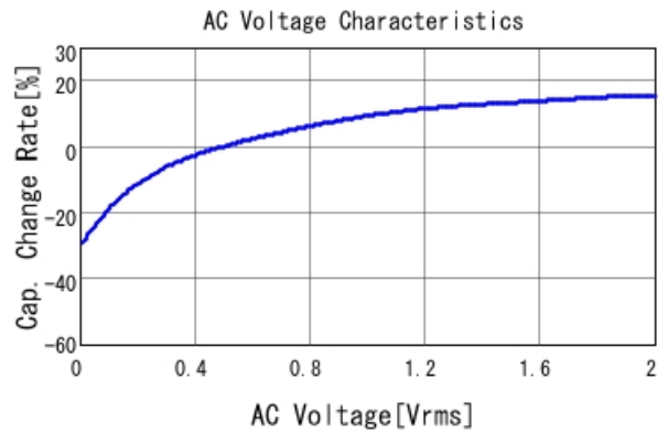
GRM185R61C105KE44 C-AC Voltage capchange, DCOV, 25
