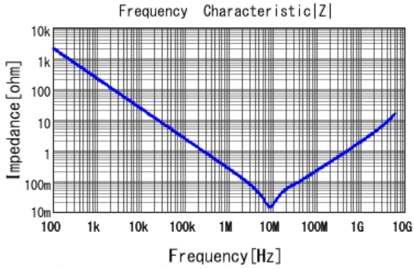
GRM185R61C105KE44 |Z| DCOV, 25degC
