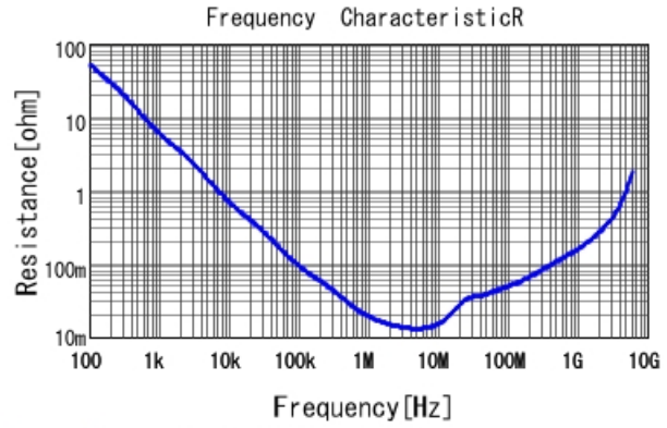
GRM185R61C105KE44 R DCOV, 25degC
