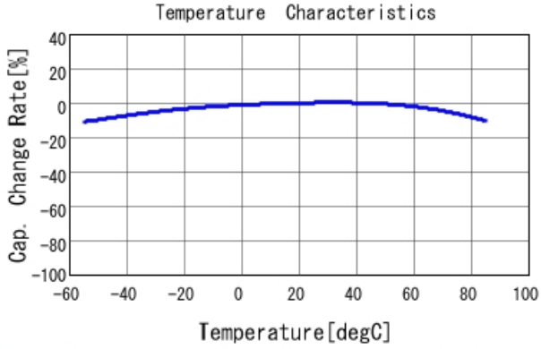
GRM185R61C105KE44 C-Temp. capchange, DC0.0V, AC0.5
