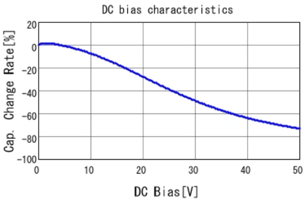
GCJ21BR71H105KA01 C-DC bias capchange, 25.0degC, A
