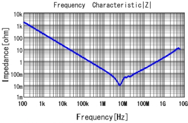
GCJ21BR71H105KA01 |Z| DCOV, 25degC
