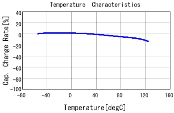
GCJ21BR71H105KA01 C-Temp. capchange, DC0.0V, AC1.C
