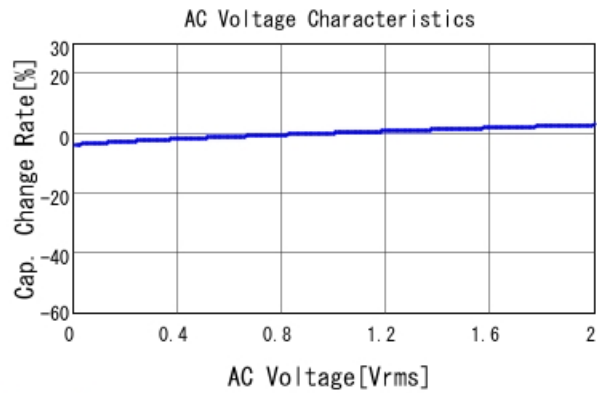
GCJ21BR71H105KA01 C-AC Voltage capchange, DCOV, 25
