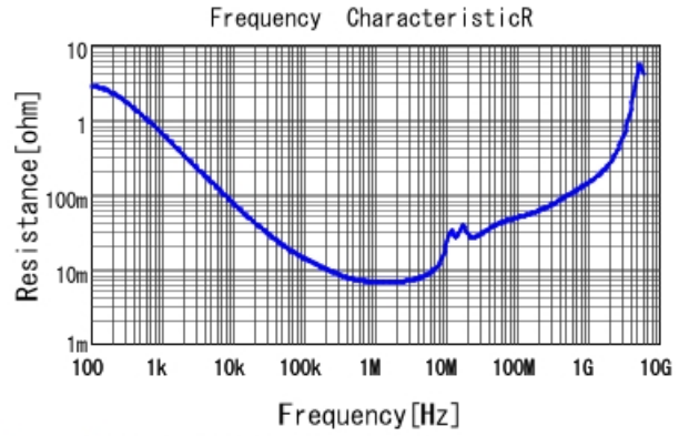
GCJ21BR71H105KA01 R DCOV, 25degC
