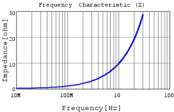
LQP02TN1N6B02 |Z|
