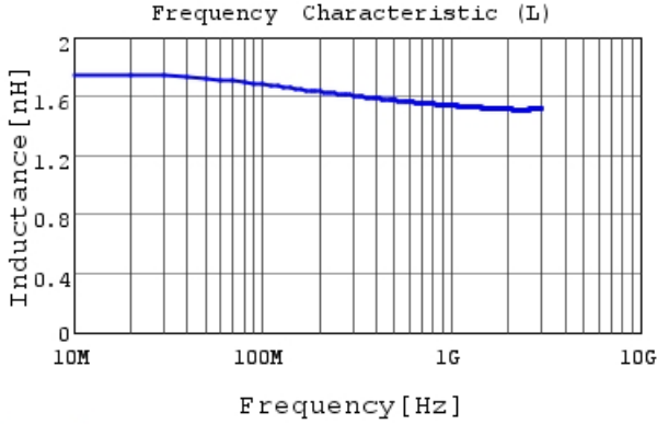
LQP02TN1N6B02 L
