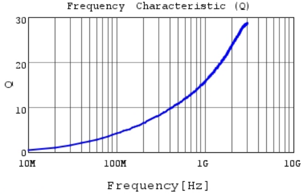
LQP02TN1N6B02 Q
