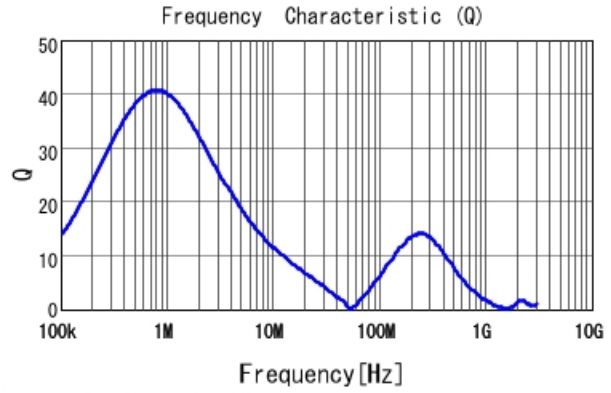
DFE2HCAH2R2MJ0 Q
