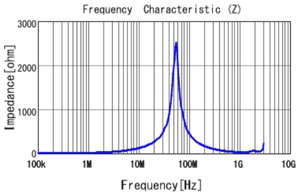
DFE2HCAH2R2MJ0 |Z|
