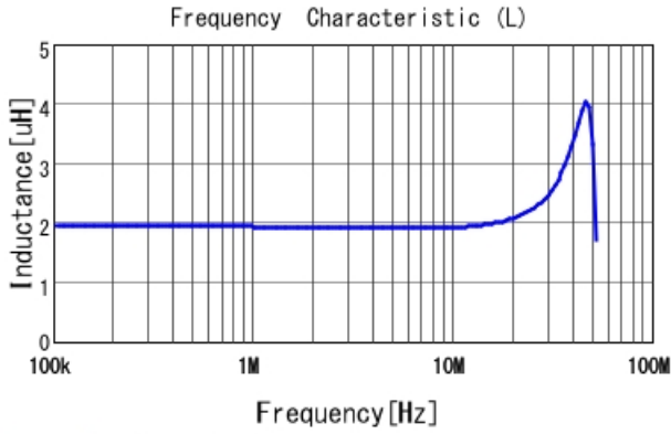
DFE2HCAH2R2MJ0 L
