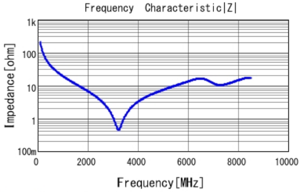
GRM1555C1H7R5DA01 |Z| DCOV, 25degC
