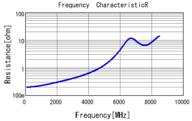
GRM1555C1H7R5DA01 R DCOV, 25degC
