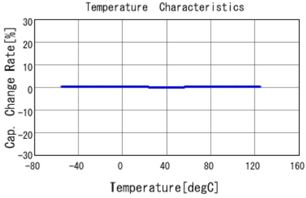
GRM1555C1H100JA01 C-Temp. capchange, DCOV, AC1Vrms
