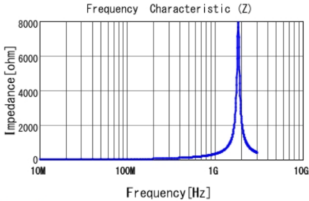
LQP03TG39NJ02 |Z|
