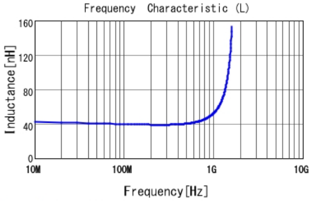
LQP03TG39NJ02 L
