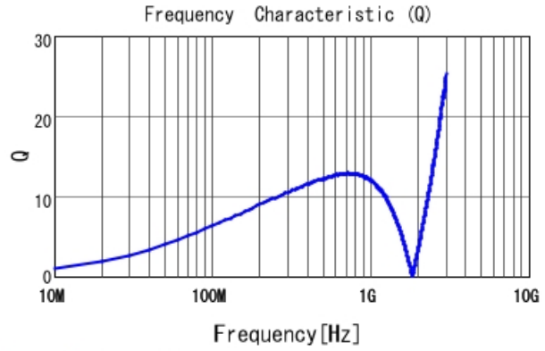
LQP03TG39NJ02 Q
