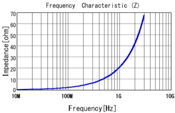
LQP03TN3N3B02 |Z|
