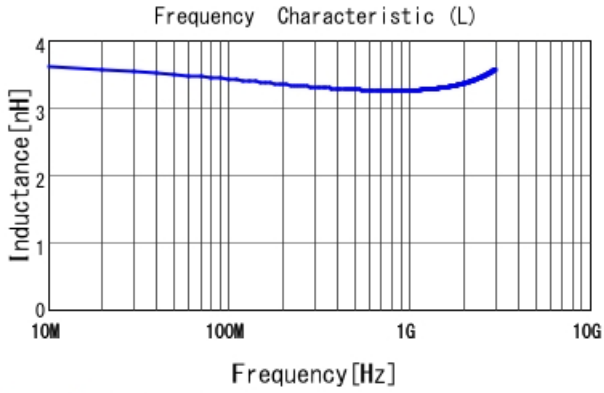
LQP03TN3N3B02 L
