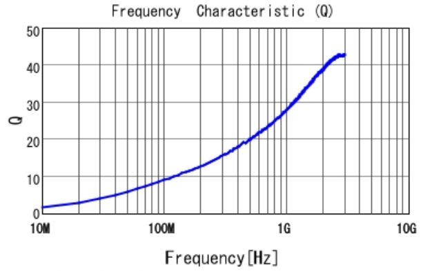
LQP03TN3N3B02 Q
