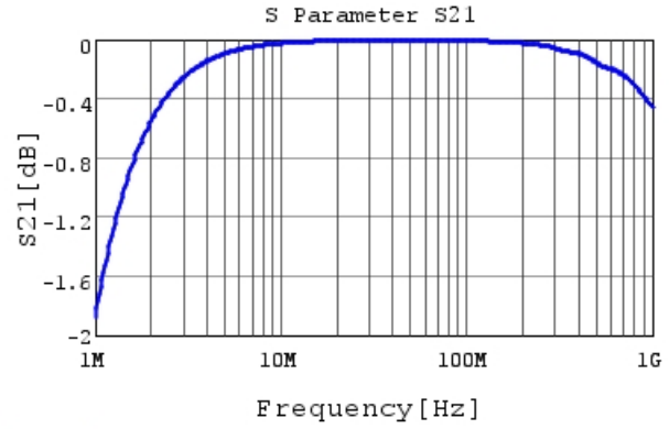
RCE5C2A222J1M1H03A S21 DC0V, 25degC
