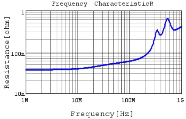
RCE5C2A222J1M1H03A R DC0V, 25degC
