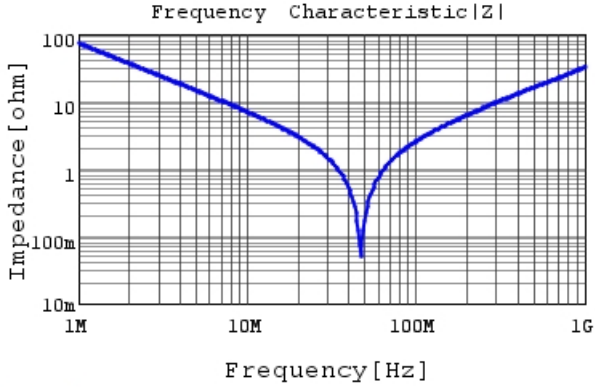
RCE5C2A222J1M1H03A |Z| DC0V, 25degC
