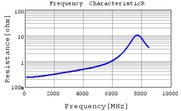
GCM1555C1H5R0FA16 R DCOV,25degC
