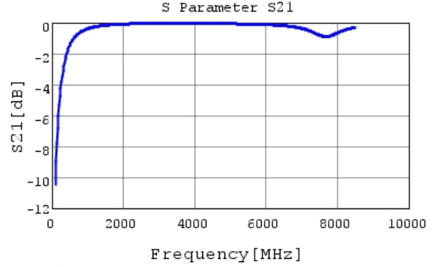
GCM1555C1H5R0FA16 S21 DCOV, 25degC
