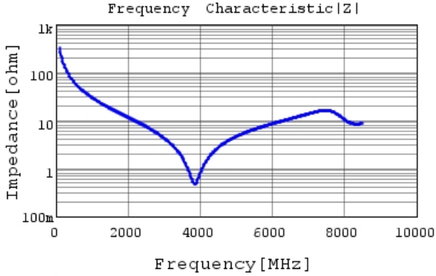
GCM1555C1H5R0FA16 |Z| DCOV,25degC
