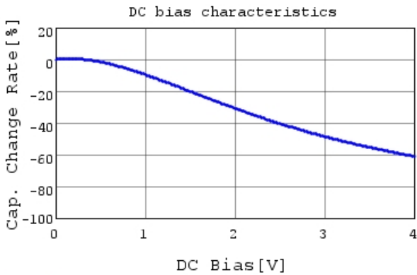
GRM188C80G106ME69 C-DC bias capchange, 25.0c
