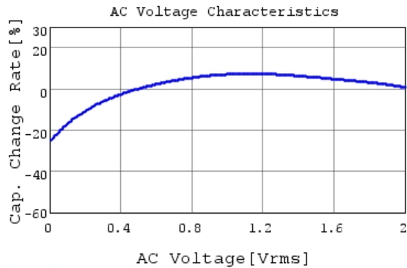
GRM188C80G106ME69 C-AC Voltage capchange, Dc
