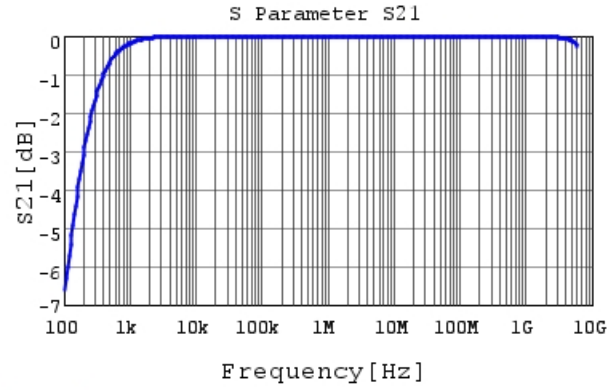
GRM188C80G106ME69 S21 DC0V,25degC
