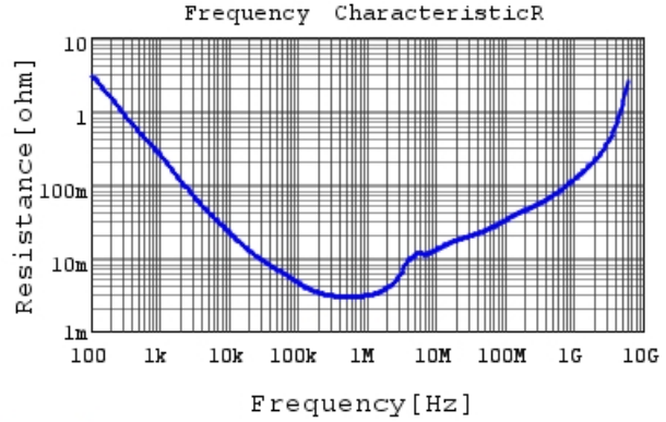
GRM188C80G106ME69 R DCOV, 25degC
