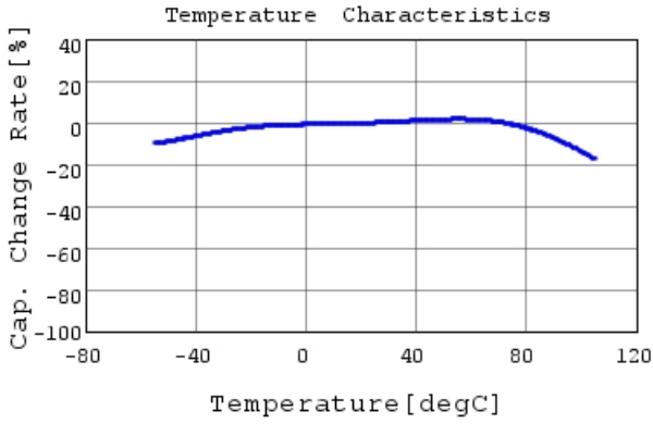
GRM188C80G106ME69 C-Temp. capchange, DC0.0V,
