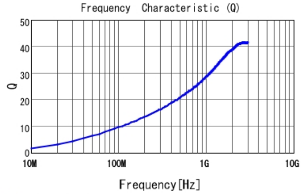
■ LQP03TN3N6C02 Q
