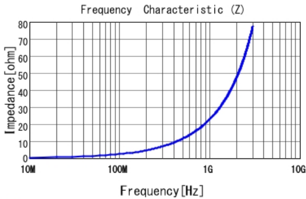
■ LQP03TN3N6C02 |Z|
