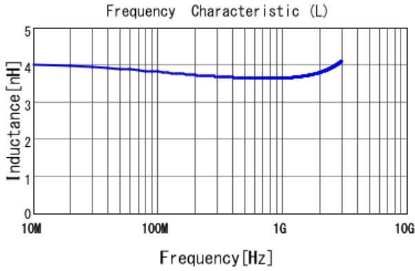
■ LQP03TN3N6C02 L
