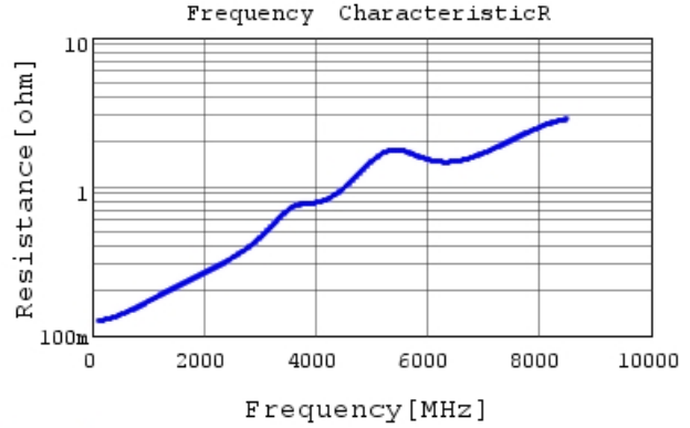
GRM0332C1H470JA01 R DCOV, 20degC
