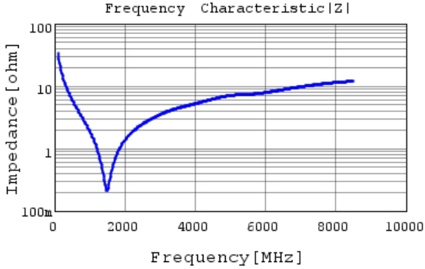
GRM0332C1H470JA01 |Z| DCOV, 20degC
