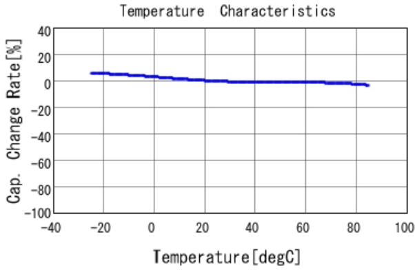
■ GRM155B31E105KA12 C-Temp. capchange, DCO. 0V, AC1. 0Vrm
