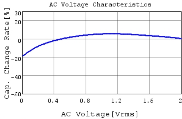
GRM033R61A224ME90 C-AC Voltage capchange, Dc
