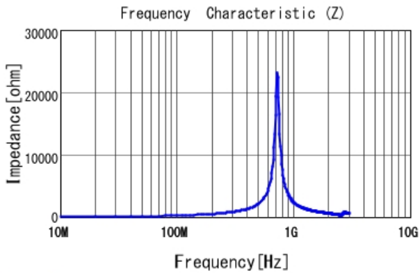
LQP03HQR39H02 |Z|
