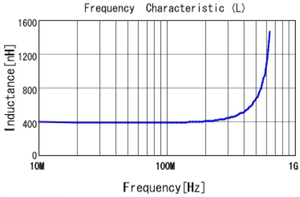
LQP03HQR39H02 L
