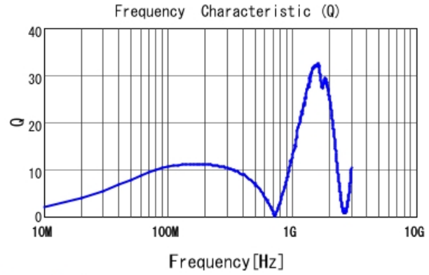
LQP03HQR39H02 Q
