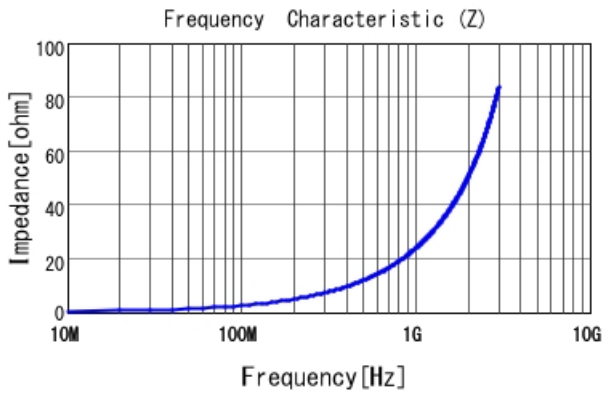
LQP03TG3N8C02 |Z|
