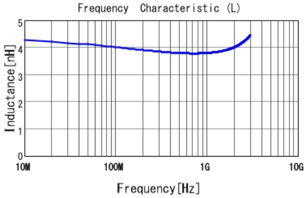
LQP03TG3N8C02 L
