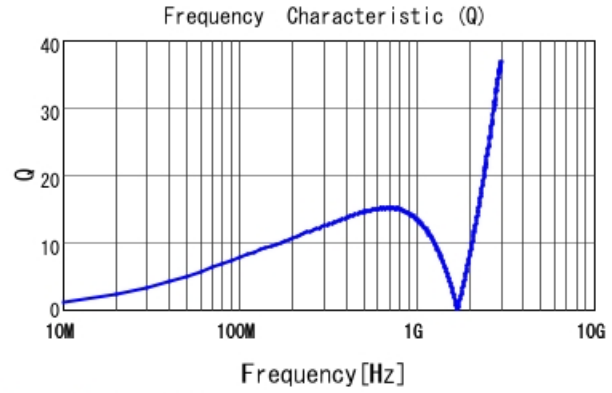
LQP03TN62NJ02 Q
