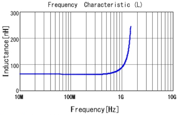
LQP03TN62NJ02 L
