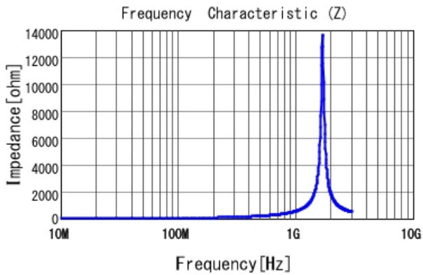
LQP03TN62NJ02 |Z|
