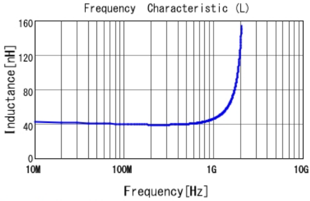
LQP03HQ39NJ02 L
