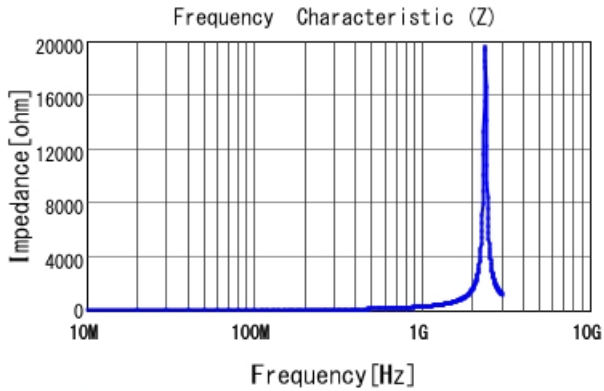
LQP03HQ39NJ02 |Z|
