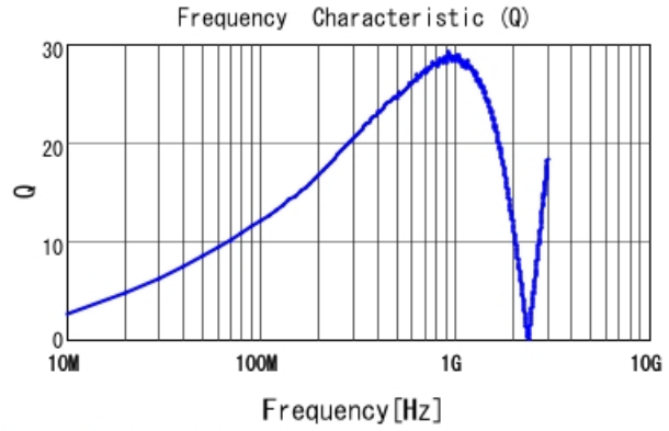
LQP03HQ39NJ02 Q
