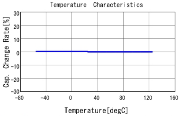
GRM3195C2A222JA01 C-Temp. capchange, DCOV, AC1Vrms
