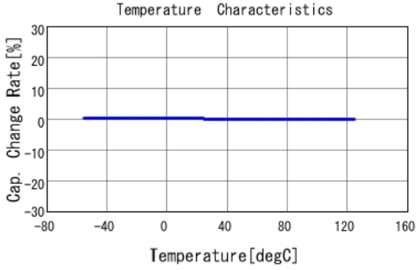
GCM2195C1H682JA16 C-Temp. capchange, DCOV, AC1Vrms
