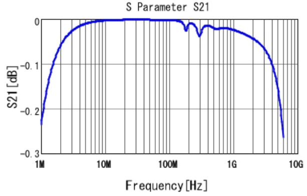
GCM2195C1H682JA16 S21 DCOV, 25degC
