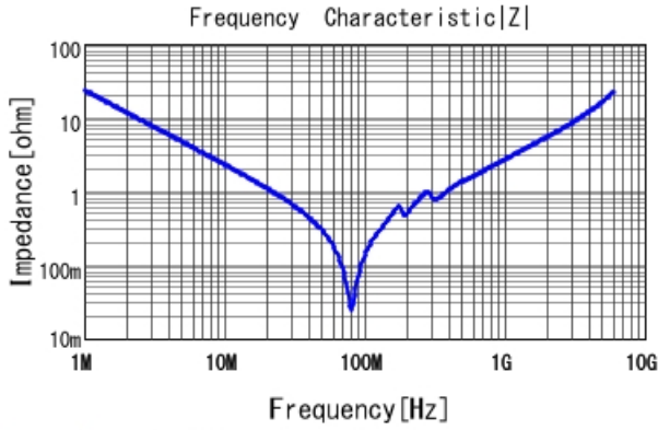
GCM2195C1H682JA16 |Z| DCOV, 25degC
