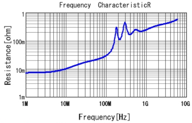
GCM2195C1H682JA16 R DCOV, 25degC
