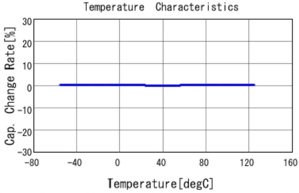
GRM1555C1H5R3BA01 C-Temp. capchange, DC0V, AC1Vrms
