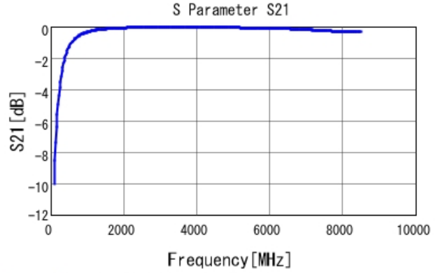
GRM1555C1H5R3BA01 S21 DC0V, 25degC
