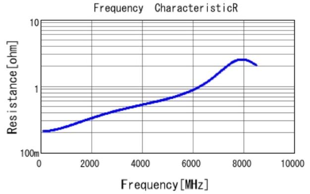
GRM1555C1H5R3BA01 R DCOV, 25degC
