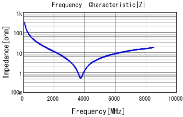
GRM1555C1H5R3BA01 |Z| DCOV, 25degC
