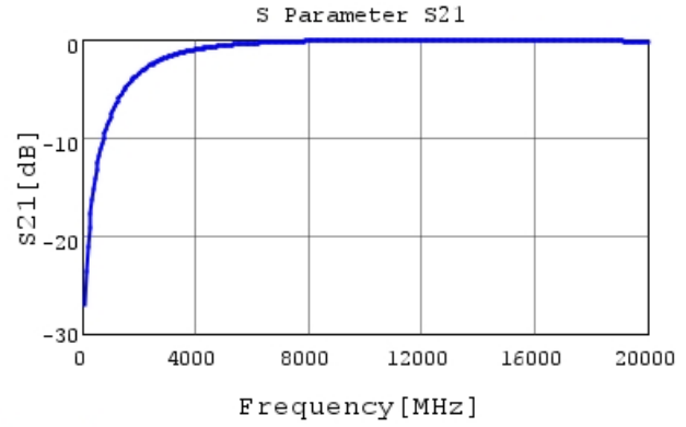
GRM0225C1ER70WA03 S21 DCOV, 25degC
