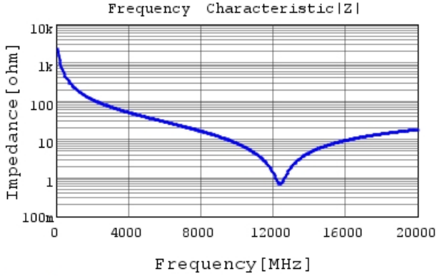
GRM0225C1ER70WA03 |Z| DCOV, 25degC
