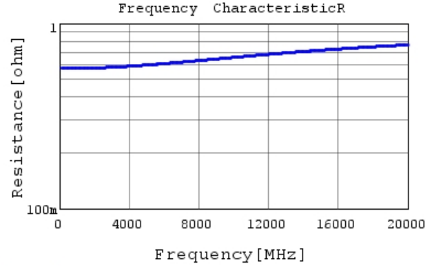
GRM0225C1ER70WA03 R DCOV, 25degC
