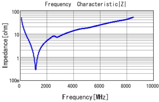
GRM1885C1H330GA01 |Z| DCOV, 25degC
