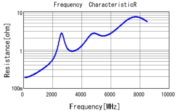
GRM1885C1H330GA01 R DCOV, 25degC
