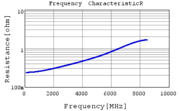
GRM0335C1H3R6CA01 R DCOV, 25degC
