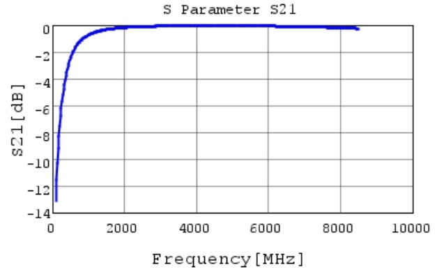
GRM0335C1H3R6CA01 S21 DCOV, 25degC
