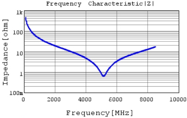
GRM0335C1H3R6CA01 |Z| DCOV, 25degC
