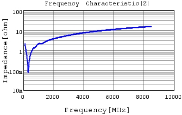
GCM1555C1H681FA16 |Z| DC0V, 25degC
