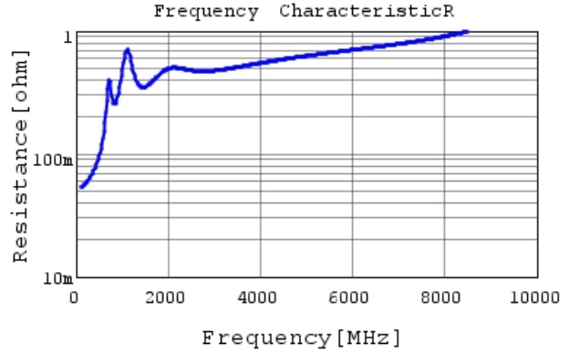
GCM1555C1H681FA16 R DC0V, 25degC
