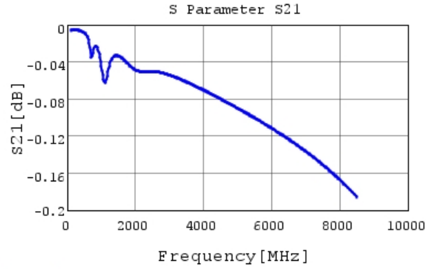
GCM1555C1H681FA16 S21 DCOV, 25degC
