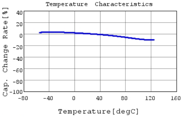
GRM033R71E182KA12 C-Temp. capchange, DC0.0V,
