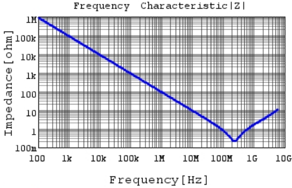
GRM033R71E182KA12 |Z| DCOV, 25degC
