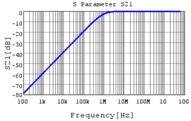
GRM033R71E182KA12 S21 DC0V, 25degC
