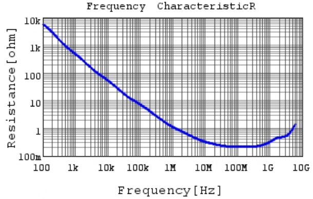
GRM033R71E182KA12 R DCOV, 25degC
