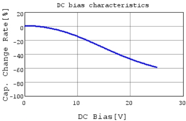
GRM033R71E182KA12 C-DC bias capchange, 25.0c
