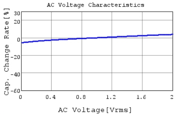
GRM033R71E182KA12 C-AC Voltage capchange, Dc
