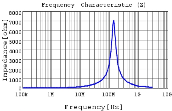
LQH2MPZ2R2MGR |Z|
