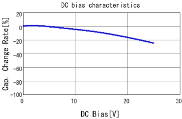
GRM188R71E473KA01 C-DC bias capchange, 25.0degC, A
