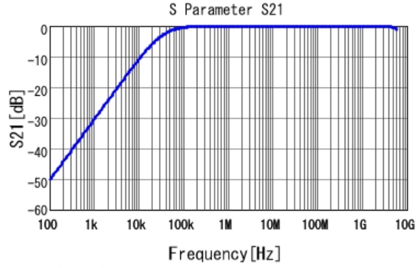
GRM188R71E473KA01 S21 DC0V, 25degC
