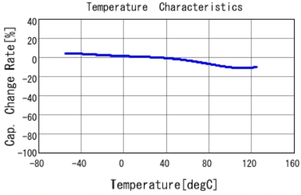
GRM188R71E473KA01 C-Temp. capchange, DC0.0V, AC1.C
