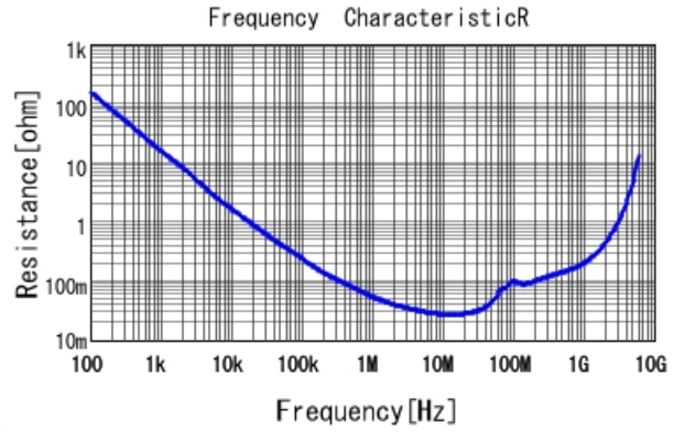
GRM188R71E473KA01 R DCOV, 25degC
