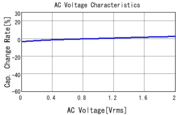
GRM188R71E473KA01 C-AC Voltage capchange, DCOV, 25
