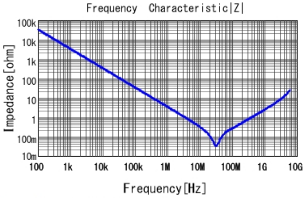
GRM188R71E473KA01 |Z| DCOV, 25degC
