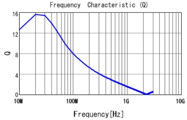
LQW04CAR12K00 Q
