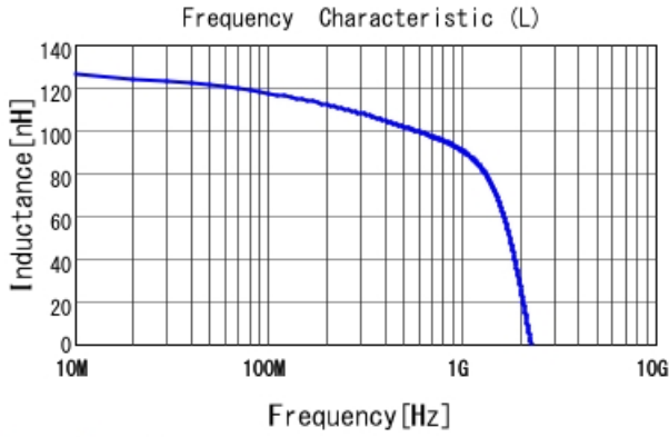
LQW04CAR12K00 L
