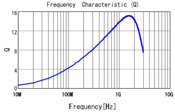
LQP02TN16NH02 Q
