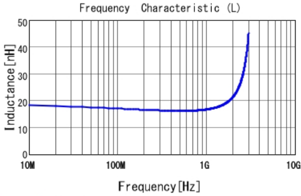
LQP02TN16NH02 L
