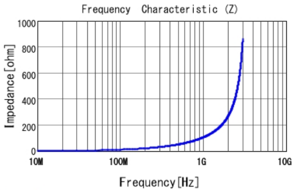
LQP02TN16NH02 |Z|
