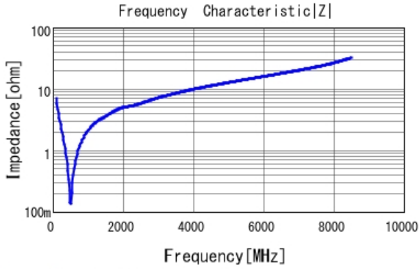
GRM1555C1H221GA01 |Z| DCOV, 25degC
