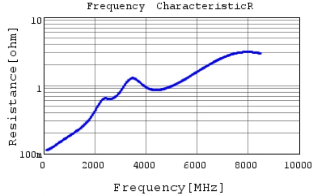
GRM0332C1H101JA01 R DCOV, 20degC
