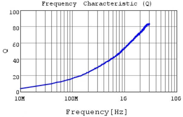
LQP03HQ2N2W02 Q
