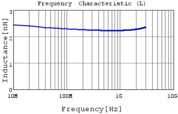
LQP03HQ2N2W02 L
