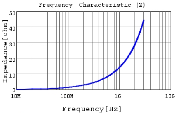
LQP03HQ2N2W02 |Z|
