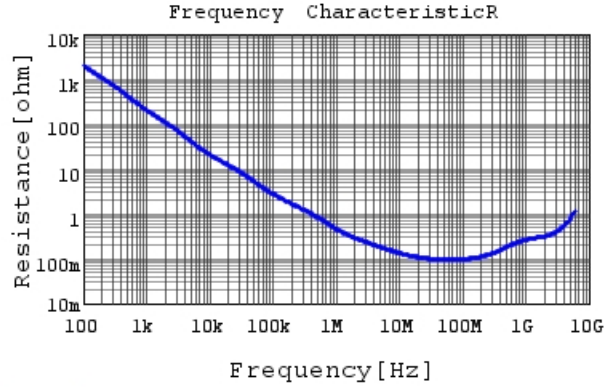
GRM033R61A472KA01 R DCOV, 25degC
