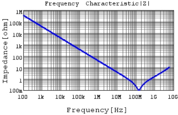
GRM033R61A472KA01 |Z| DCOV, 25degC
