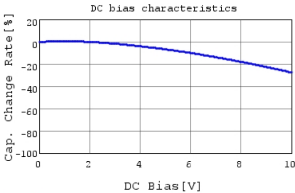
GRM033R61A472KA01 C-DC bias capchange, 25.0c
