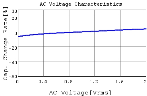
GRM033R61A472KA01 C-AC Voltage capchange, Dc
