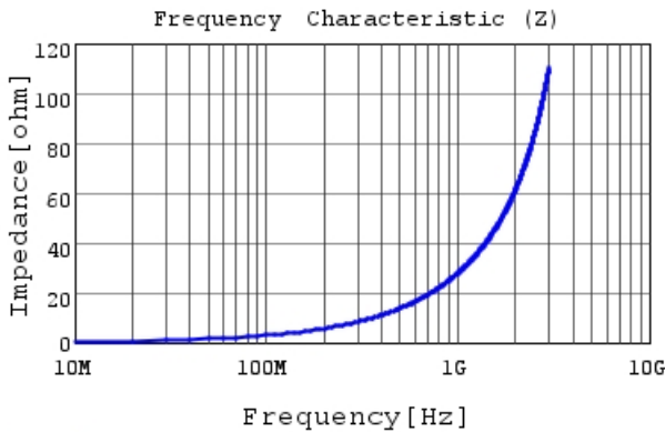
LQG15HS4N7S02 |Z|
