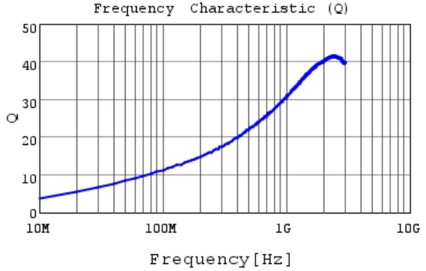
LQG15HS4N7S02 Q
