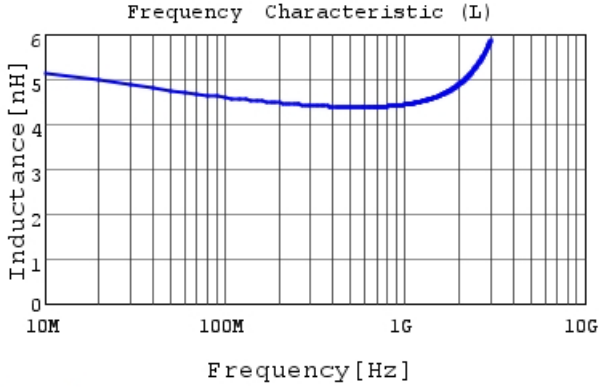
LQG15HS4N7S02 L
