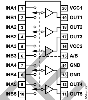
Figure 5. Pin Configuration, ADD8505, 5-Channel Buffer
