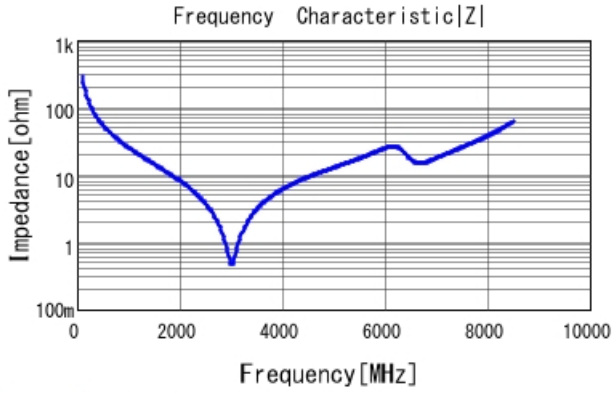
GRM1885C1H5R6BA01 |Z| DCOV, 25degC
