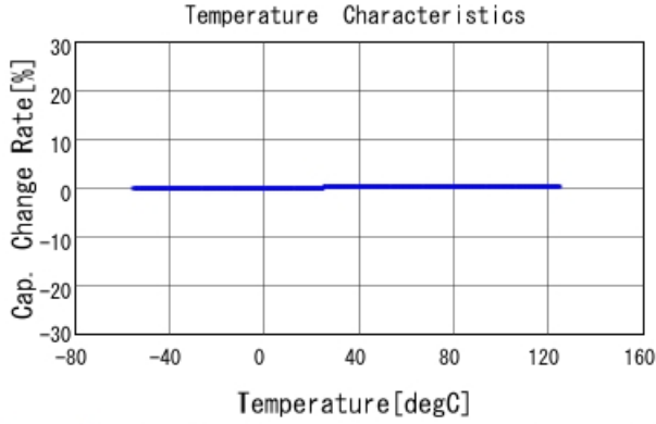
GRM1885C1H5R6BA01 C-Temp. capchange, DCOV, AC1Vrms
