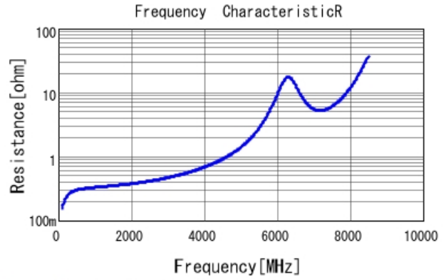
GRM1885C1H5R6BA01 R DCOV, 25degC
