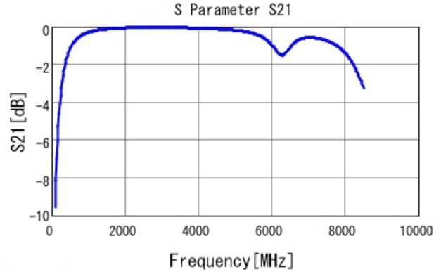
GRM1885C1H5R6BA01 S21 DCOV, 25degC
