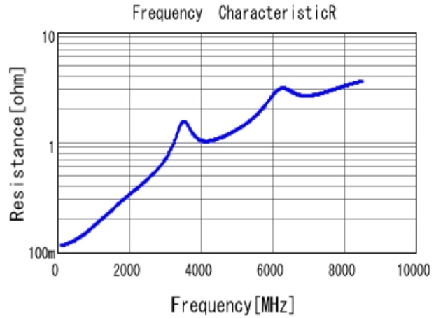
■ GRM1555C1H270JA01 R DC0V, 25degC
