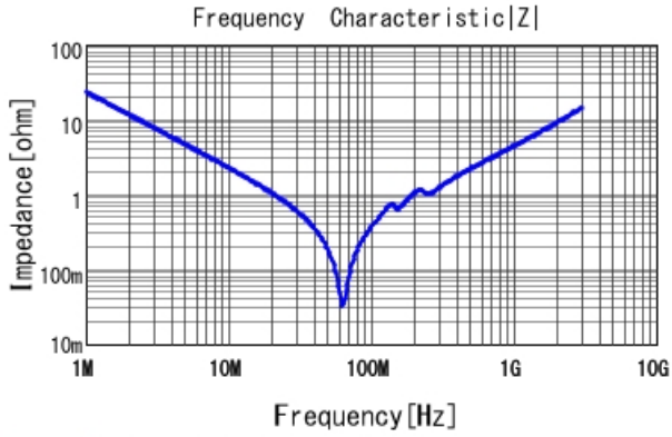
GRM31B7U2E682JW31 |Z| DCOV, 25degC
