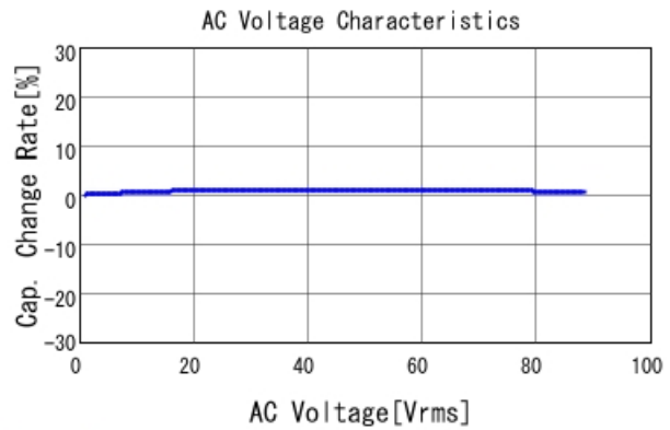
GRM31B7U2E682JW31 C-AC Voltage capchange, DCOV, 25
