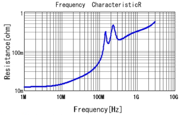
GRM31B7U2E682JW31 R DCOV, 25degC
