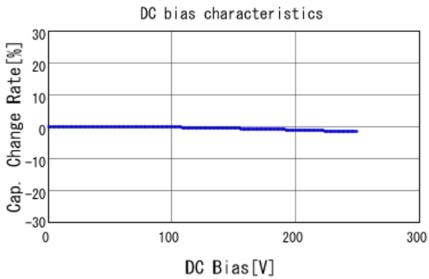
GRM31B7U2E682JW31 C-DC bias capchange, 25.0degC, A
