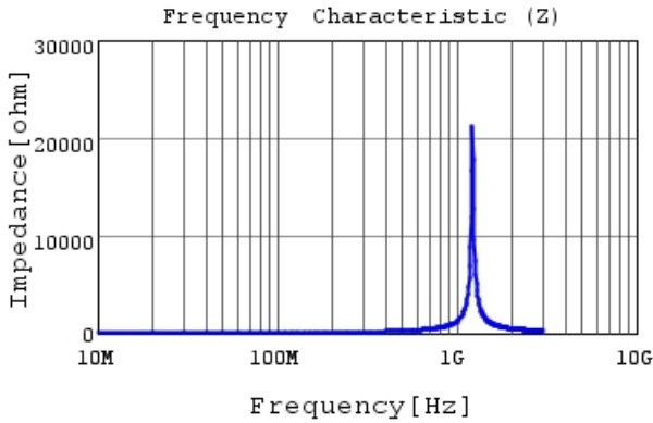
LQG18HH68NJ00 |Z|
