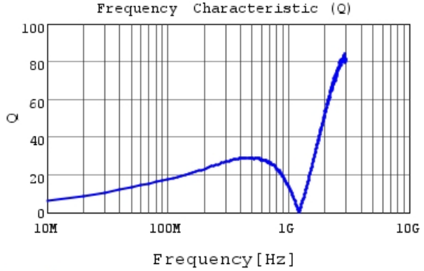
LQG18HH68NJ00 Q
