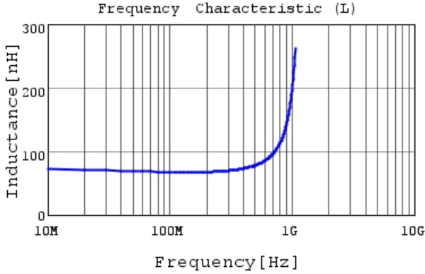
LQG18HH68NJ00 L
