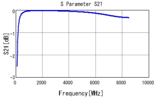
GRM0335C1E180JA01 S21 DCOV, 25degC
