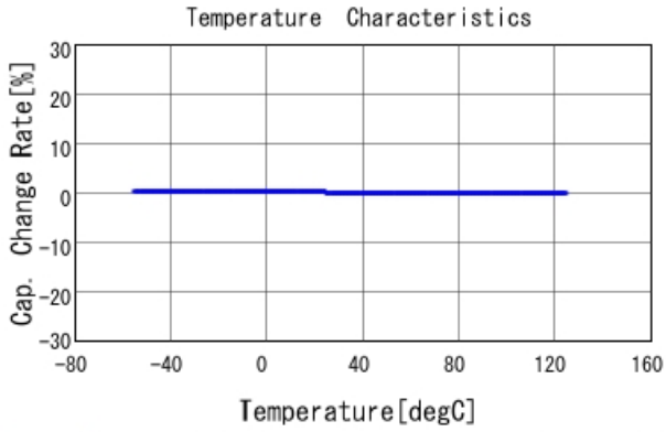
GRM0335C1E180JA01 C-Temp. capchange, DCOV, AC1Vrms
