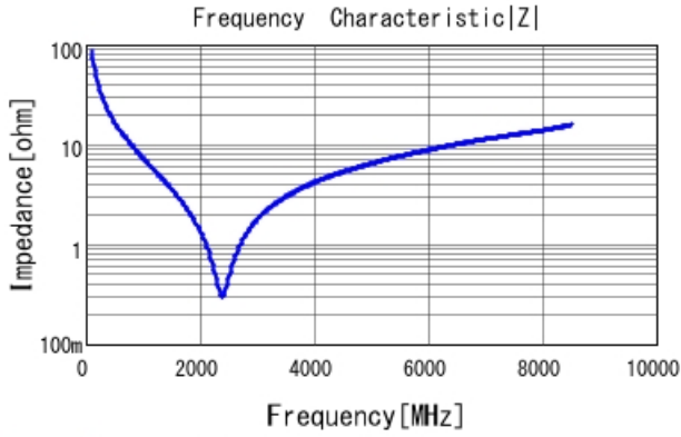
GRM0335C1E180JA01 |Z| DCOV, 25degC
