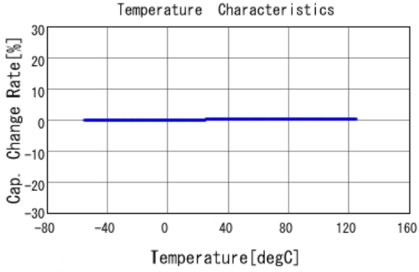
GRM1885C1H4R7CA01 C-Temp. capchange, DCOV, AC1Vrms
