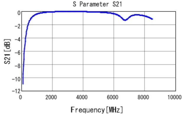
GRM1885C1H4R7CA01 S21 DCOV, 25degC
