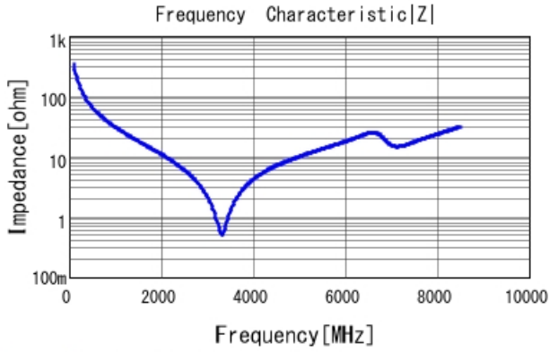
GRM1885C1H4R7CA01 |Z| DCOV, 25degC
