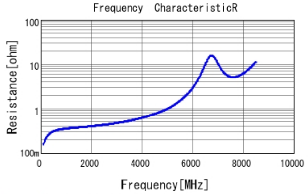
GRM1885C1H4R7CA01 R DCOV, 25degC
