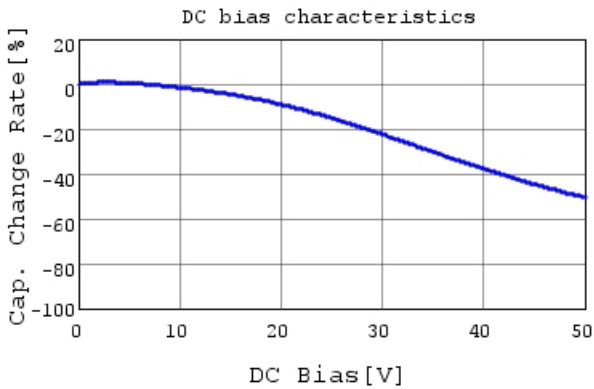
GCM188L81H104KA57 C-DC bias capchange, 25.0c
