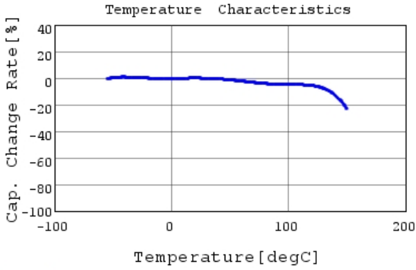
GCM188L81H104KA57 C-Temp. capchange, DC0.0V,
