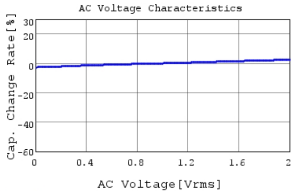
GCM188L81H104KA57 C-AC Voltage capchange, Dc
